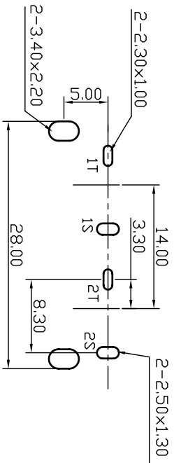
Pin Hole Layout (Jack Bottom View)
