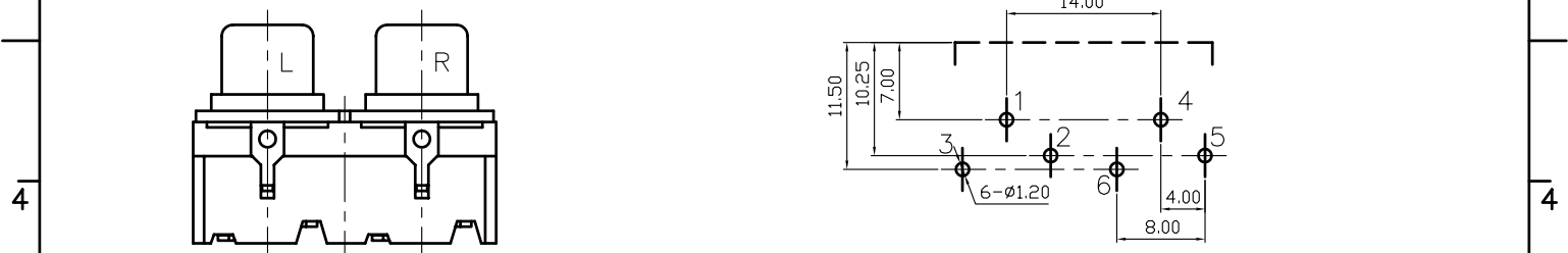
Pin Hole Layout (Jack Bottom View)
