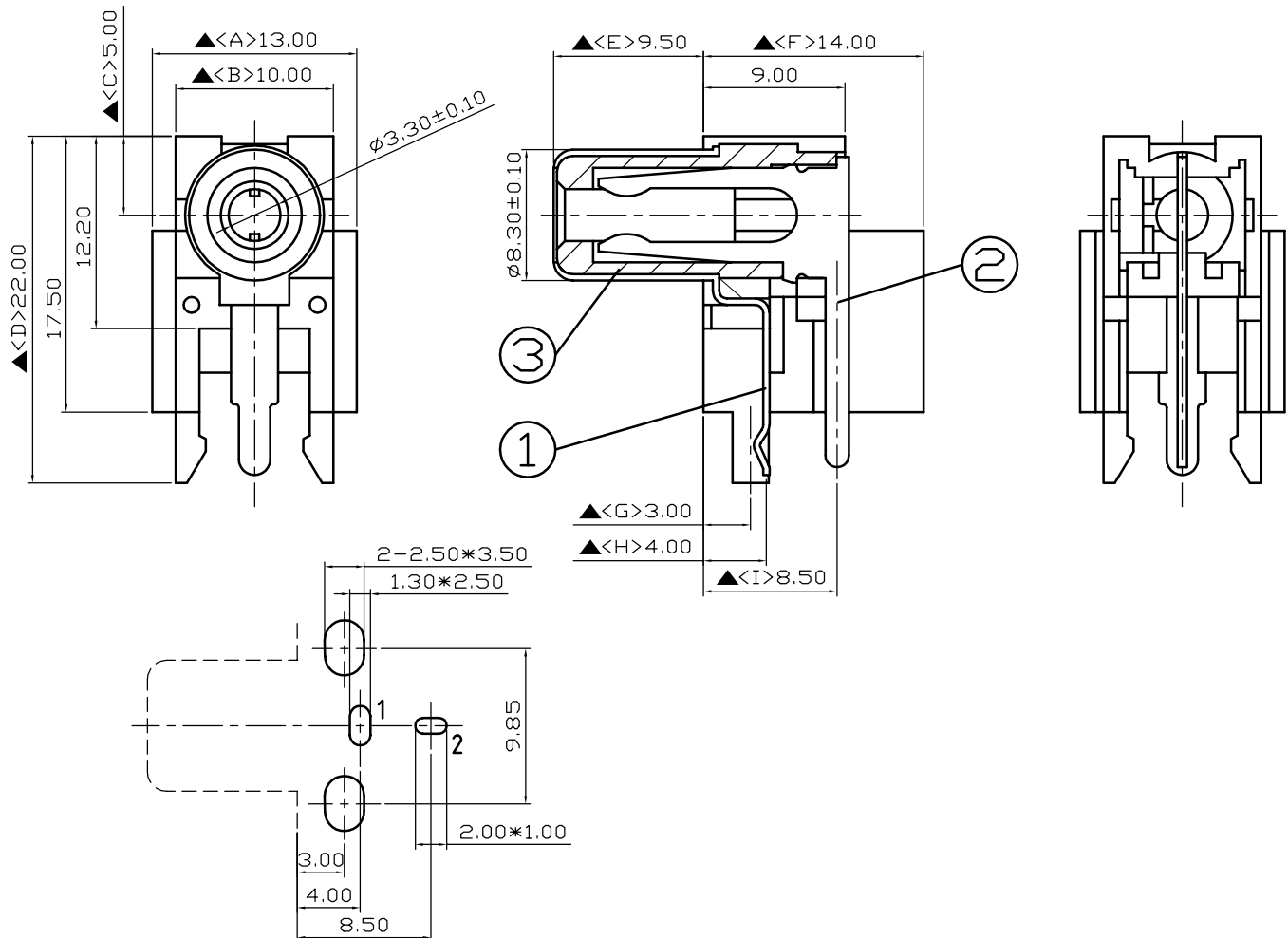
Pin Hole Layout (Jack Bottom View)
